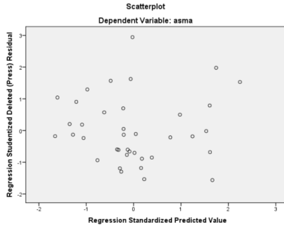
Gambar 4. Scatterplot
