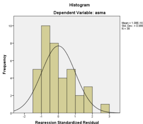
Gambar 1. Distribusi Histogram
